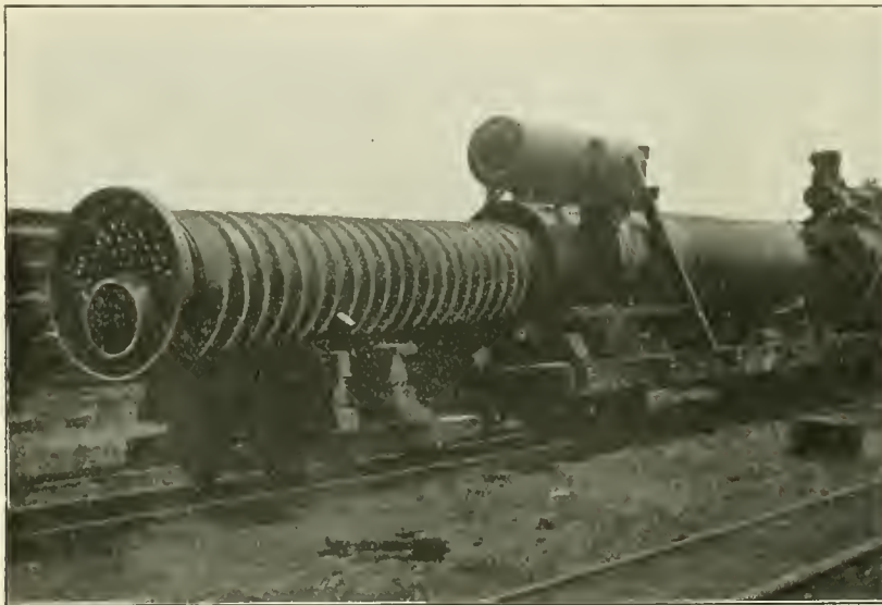
THOMAS & STETSON OIL-BURNING LOCOMOTIVE.
